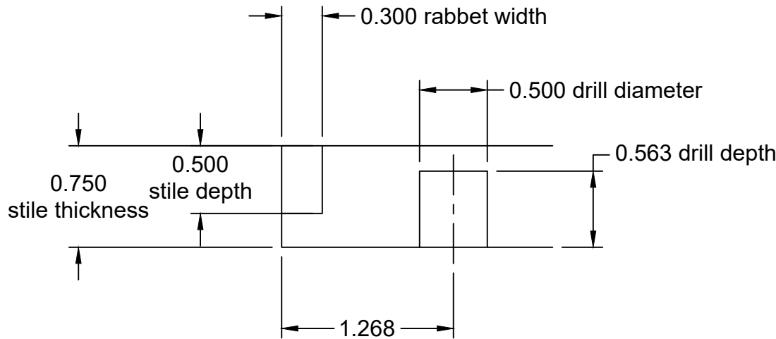
TYPICAL DETAIL
